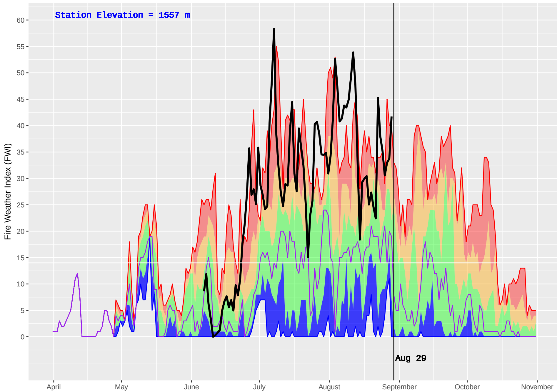
SKOONKA (1024) : Historical (2008–2016) and Current (2017) Noon Fire Weather Index (FWI)
