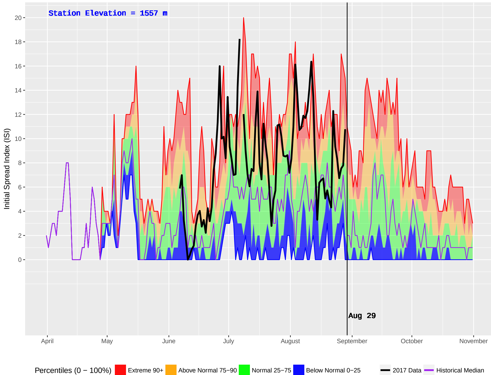
SKOONKA (1024) : Historical (2008–2016) and Current (2017) Noon Initial Spread Index (ISI)
